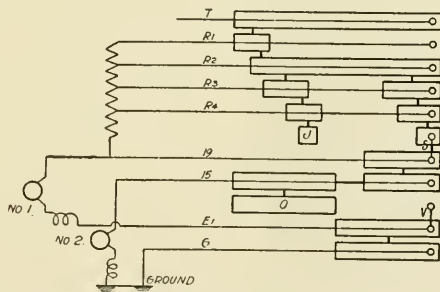
Fig. 54. Development of Controller Connections—Motors in Parallel
